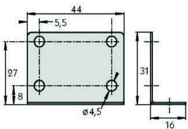
Fixing Bracket
