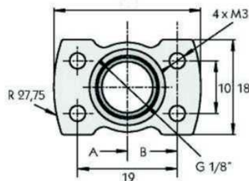
Adapter Flange
