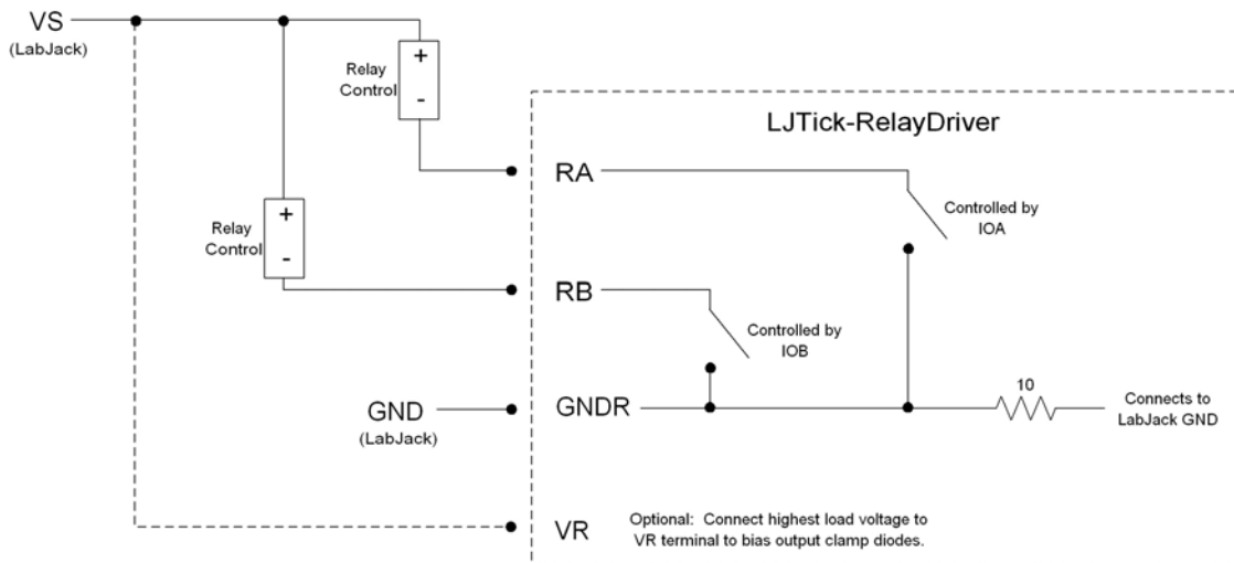
Figure 5: Connection Diagram When Controlling VS from LabJack
