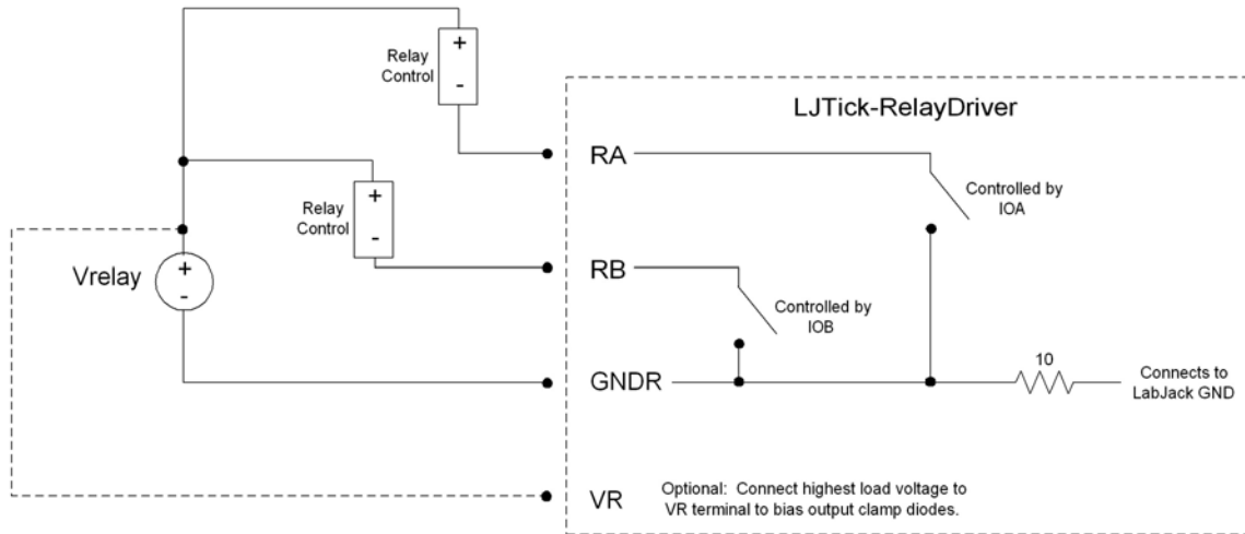
Figure 4: General Connection Diagram
